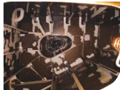
Sea Water Ballast Tank Coal-tar Epoxy Repair
