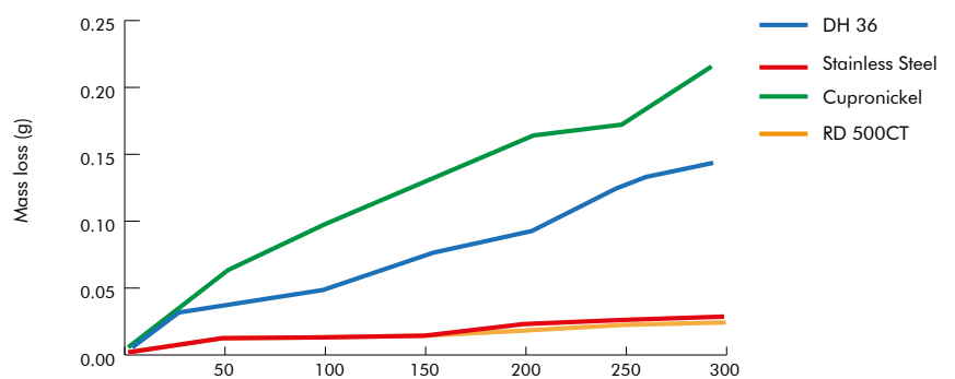
Fresh Water, 1mm gap, 75% Power (750W), -790 mV CP
